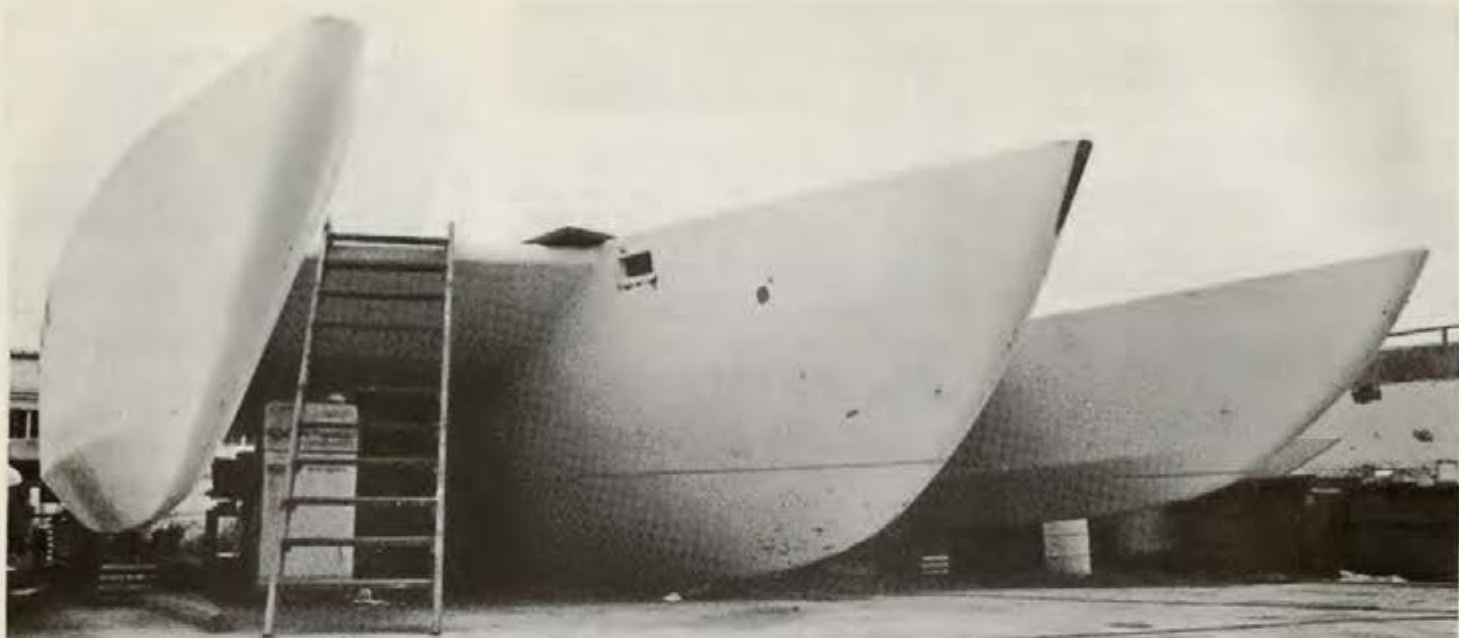
With overall length of 56' and beam of 32', this trimaran will be ketch rigged with a sail plan for 1,300 sq. ft. of working sail and 4,000 sq. ft. for racing.
